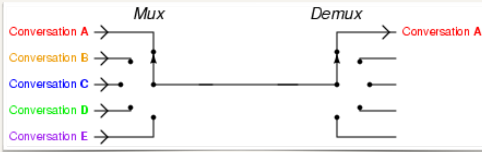
Fig 2.18. - Multiplexage temporel
